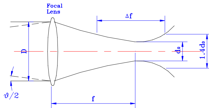
Figure 6: Focusing of a Gaussian beam
