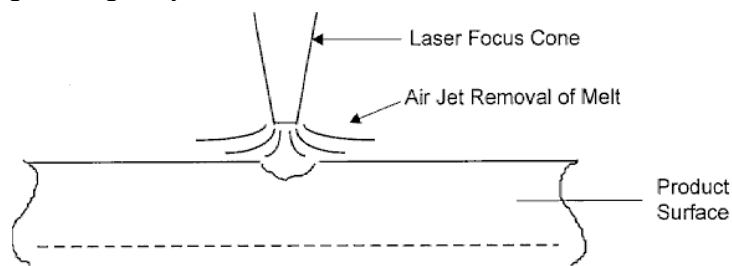
Figure 3: Softening and melting marking
